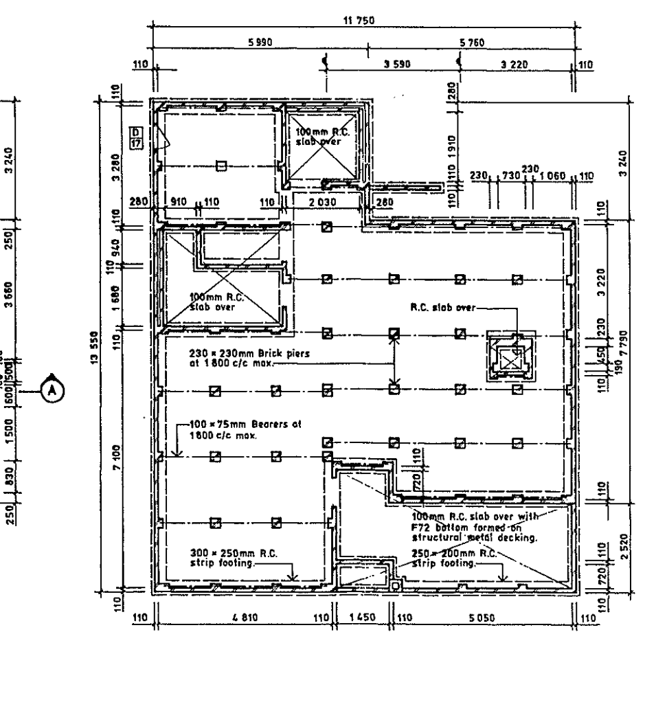
FOUNDATION PLAN SCALE 1:100
